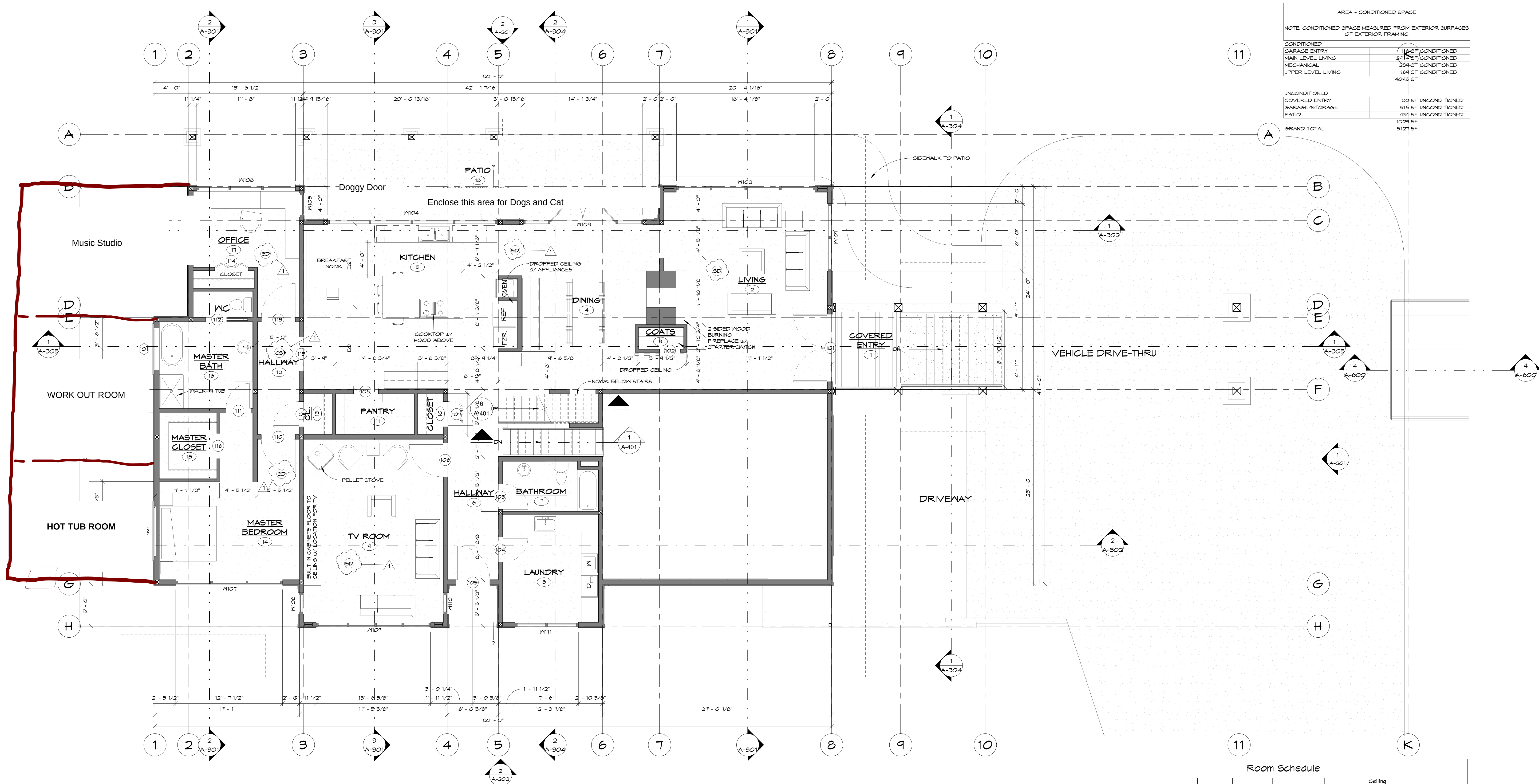
1 MAIN LEVEL 3/16" = 1'-0"
