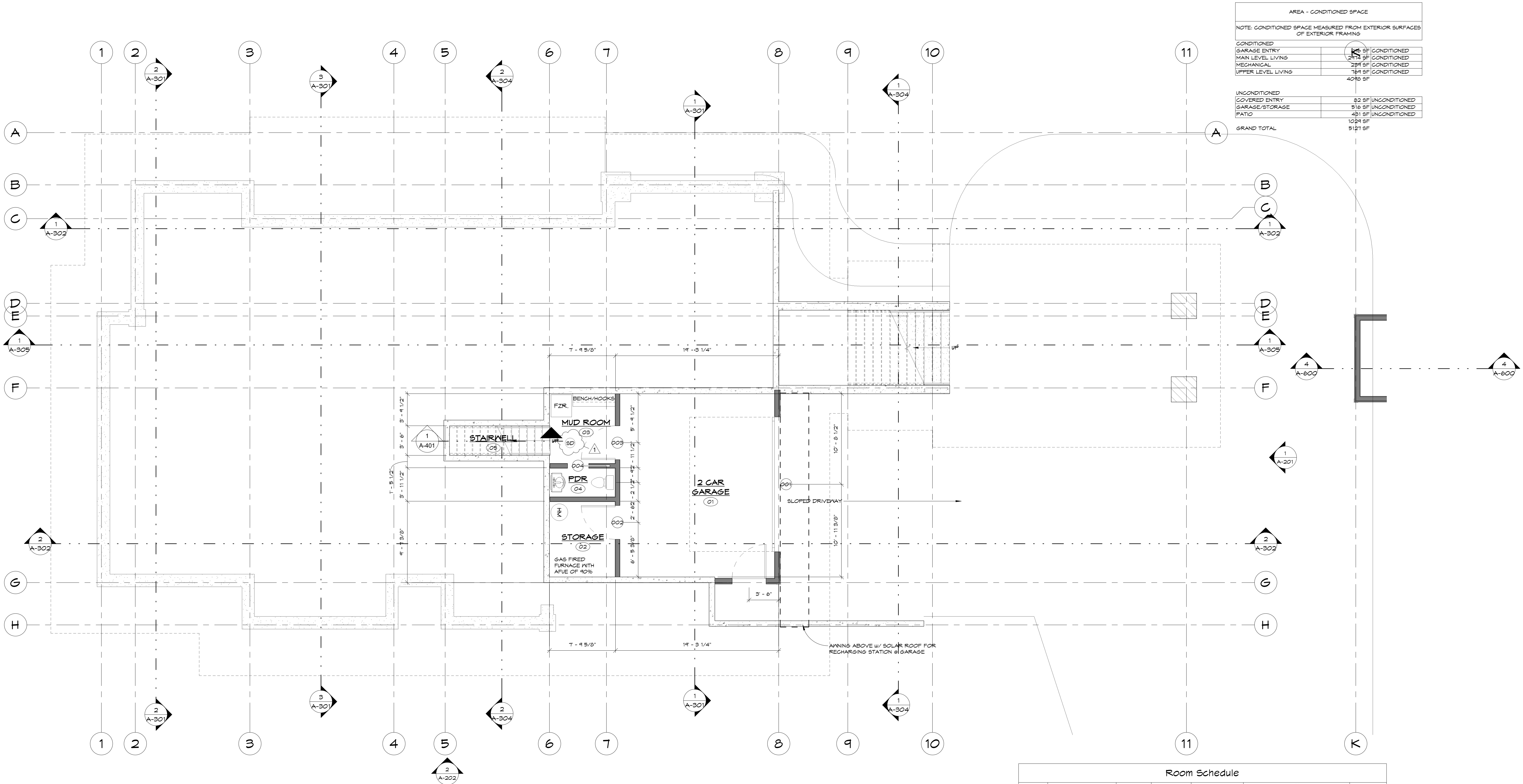
1 GARAGE LEVEL 3/16" = 1'-0"
