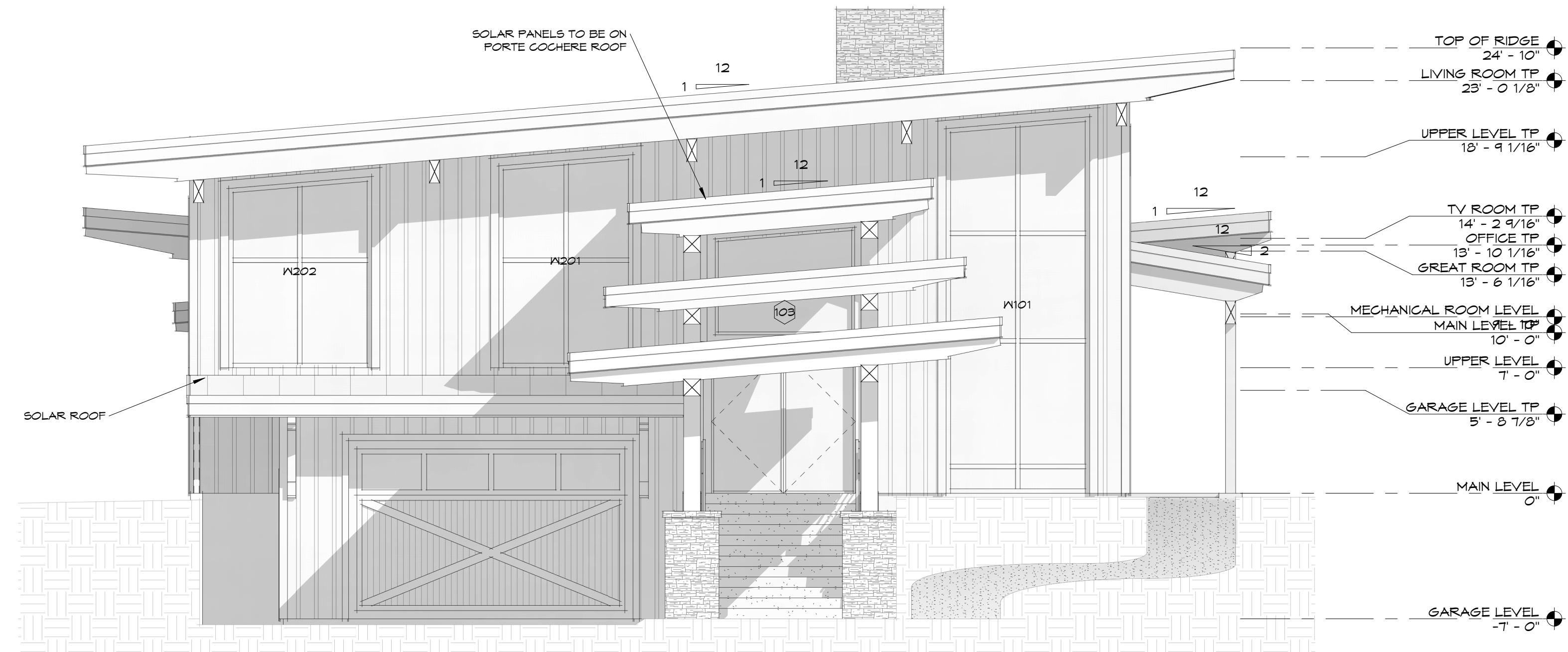
1 FRONT (SOUTH) 3/16" = 1'-0"
