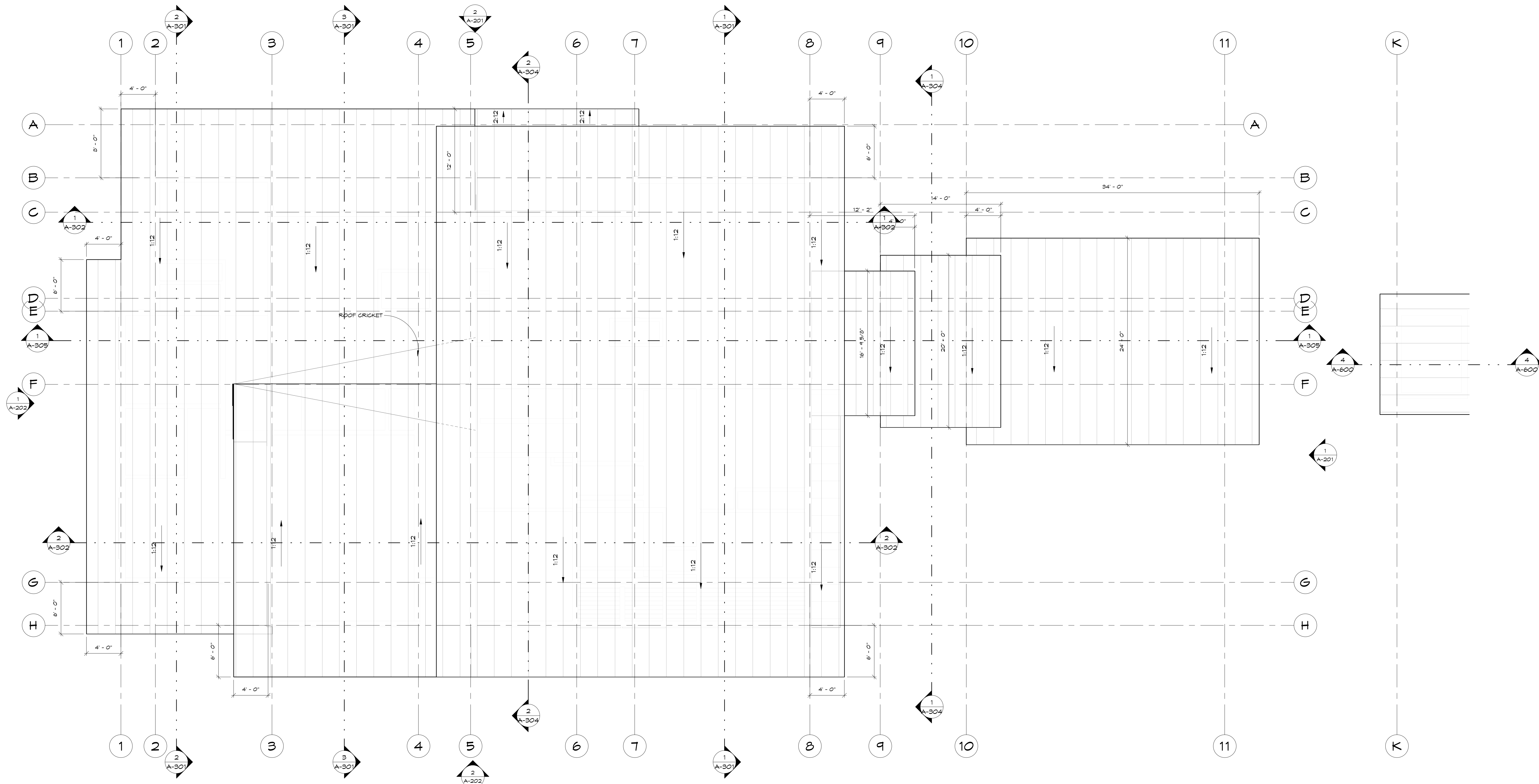
1 ROOF PLAN 3/16" = 1'-0"
