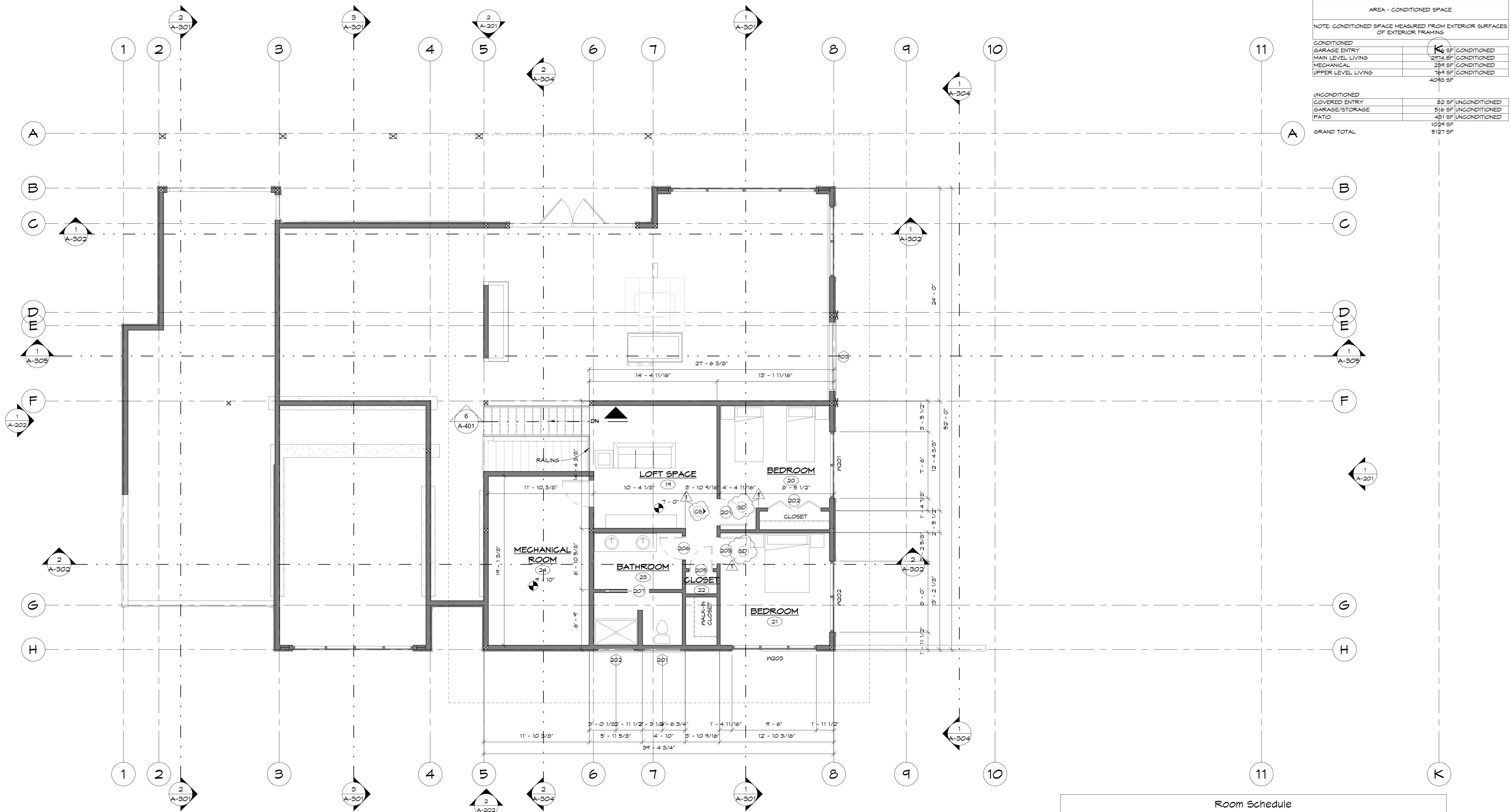
1 UPPER LEVEL 3/16" = 1'-0"
