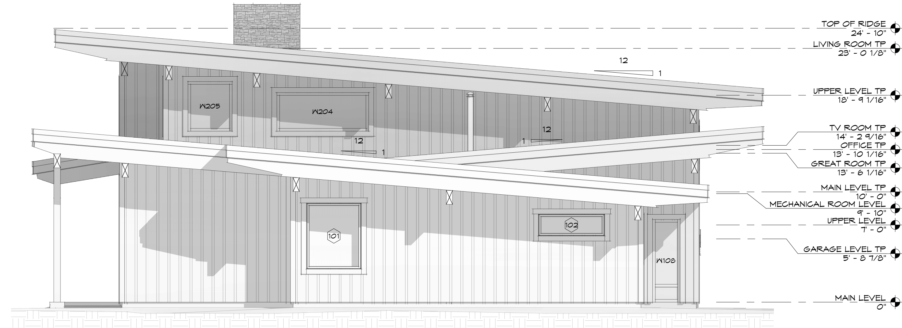
1 REAR (NORTH) 3/16" = 1'-0"
